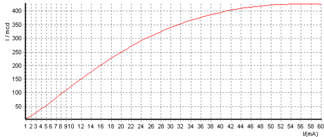
电流-光强曲线 Current-Luminous intensity Curve
